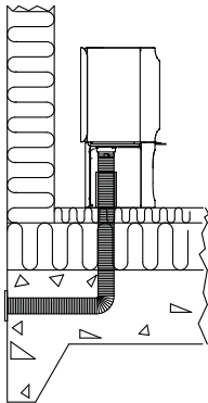
Fig. 2C, through the floor and basement
